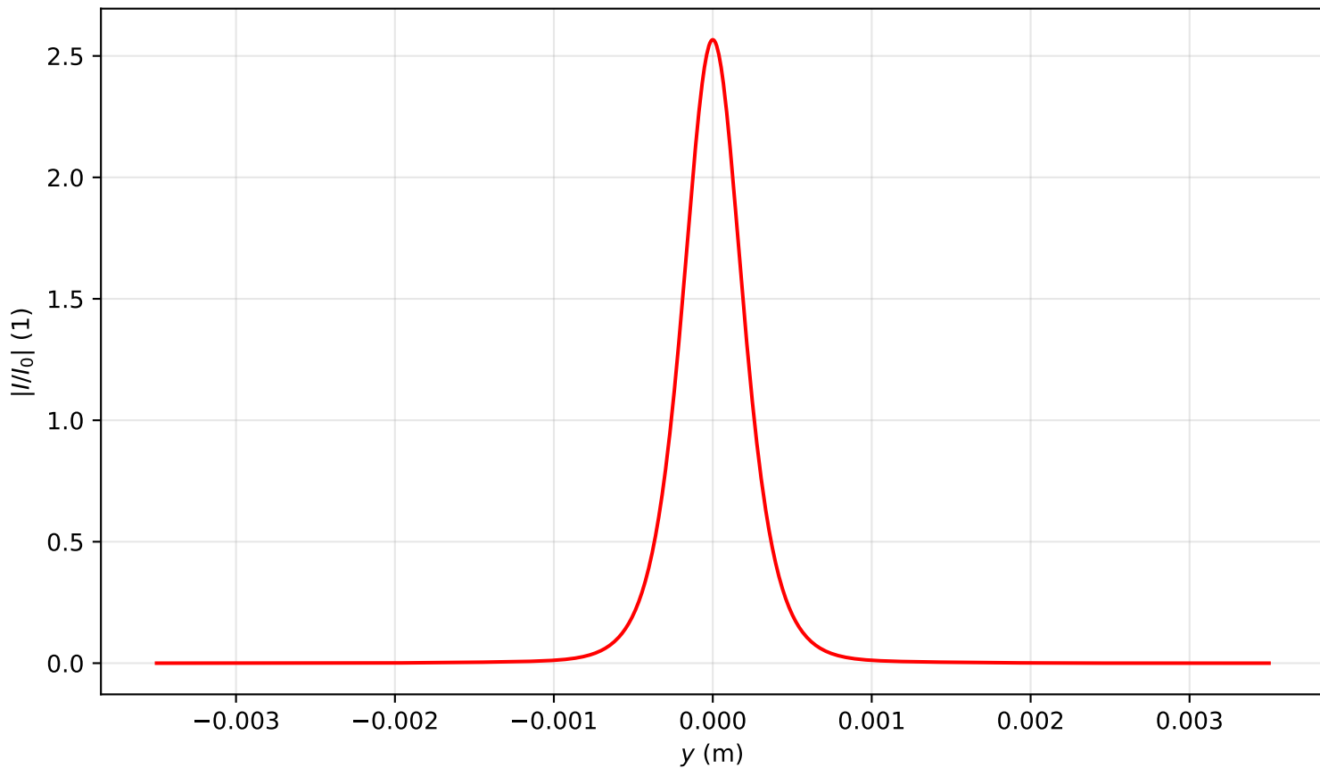
Intensity profile I(x=0, y, z=2.866)/I_0 , \text{Pin}=1.0\text{Pcr} , artificial time
